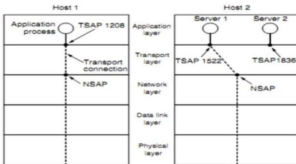
TSAP and NSAP network connections
