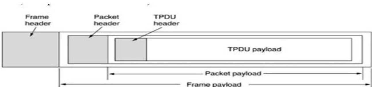
Nesting of TPDUs, Packets, and Frames
